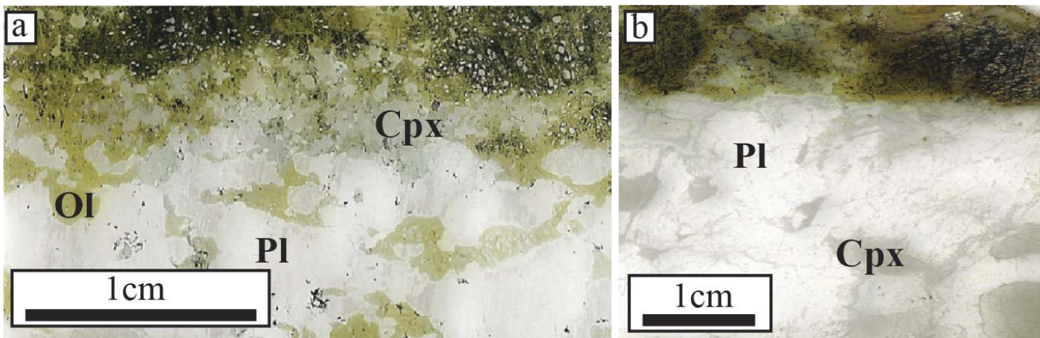
Fig. 34 - Stop 5.2, a, b) Thin section images: a) diffuse contacts between an olivine-gabbro and mantle peridotites; b) sharp-planar contacts between a clinopyroxene-rich and the mantle peridotites. OI, Olivine; Pl, plagioclase; Cpx, clinopyroxene.
