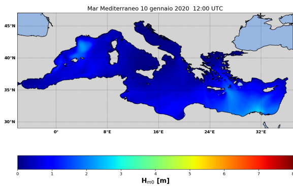
(a) ore 12 UTC 10/01/2020
