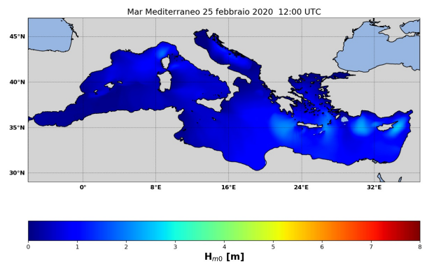
(b) ore 12 UTC 25/02/2020
