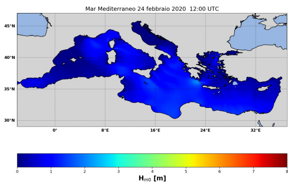
(a) ore 12 UTC 24/02/2020
