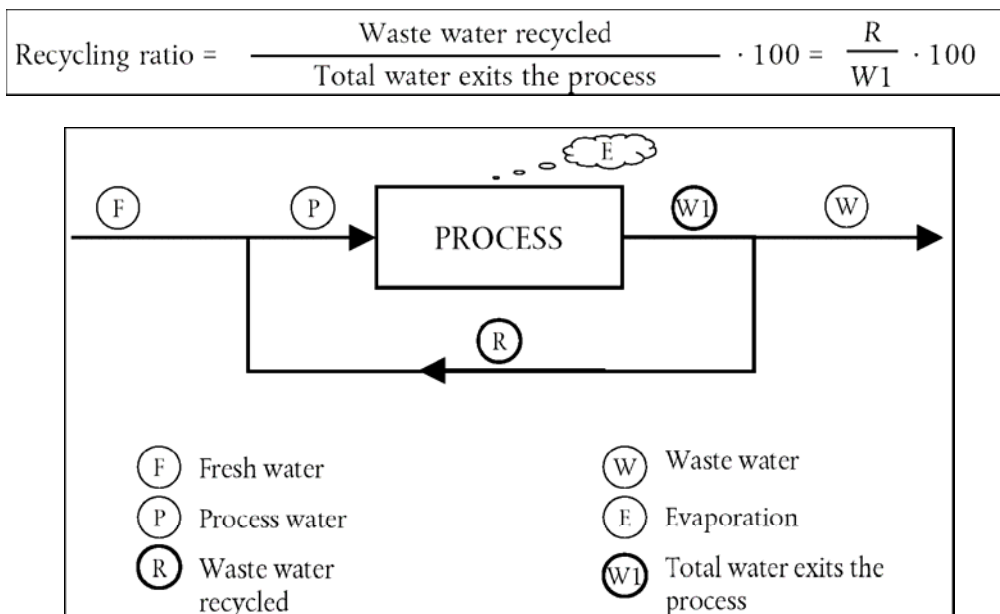
Figure A2: Water flow scheme that shall be used to calculate Water Recycling Ratio 16
