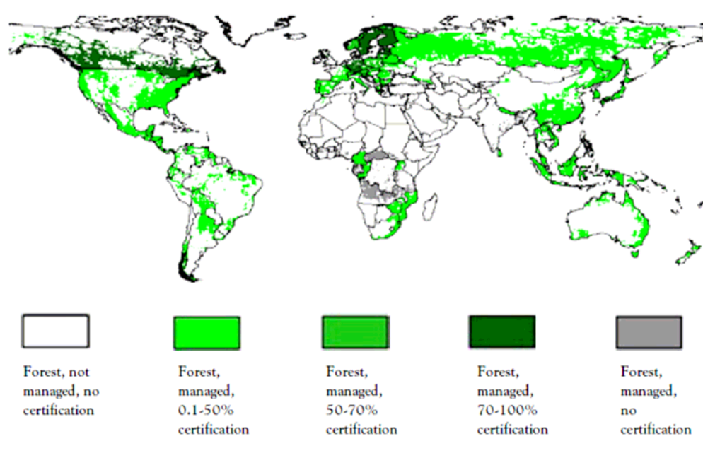
Figure 3.1 - Forest area certified relative to the forest area under management by countries. It is assumed that managed forest is at least 55% influenced by human activity. (Source: UNECE, 2008)
