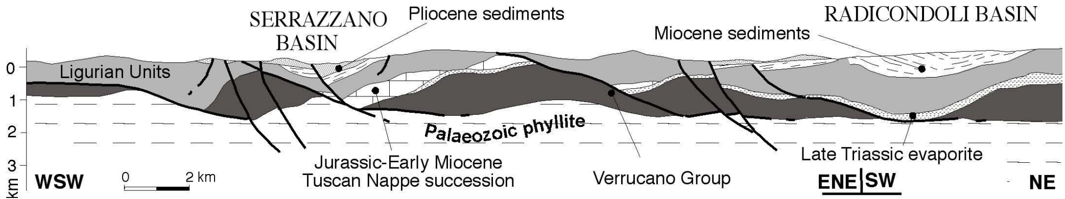
Fig. 2.8 - Geological cross section through the Larderello area and surroundings based on borehole stratigraphy, seismic reflection lines and field mapping, showing the lateral segmentation of the Tuscan Nappe and Verrucano Group (after Brogi and Liotta, 2008).
