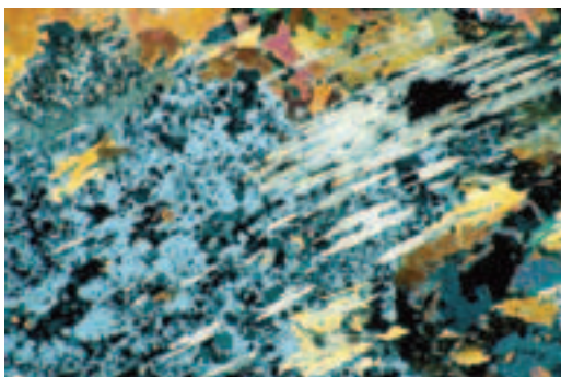
Figure 36 - The reaction of staurolite to hercynite accompanies the topotactic replacement of andalusite by sillimanite in the metapelites at Stop 2. Taken from Cesare (1994a).
