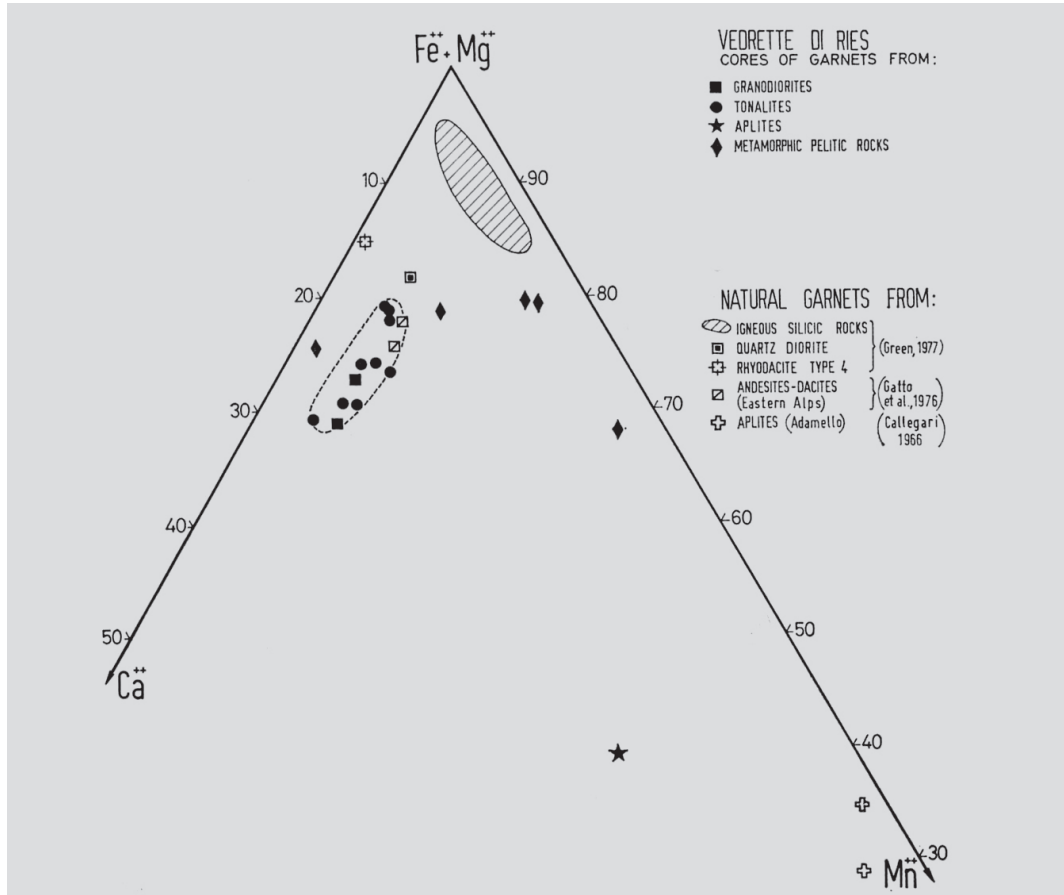
Fig. 8. Composition of the cores of the garnets studied and of some garnets known in the literature (GREEN, 1977).
