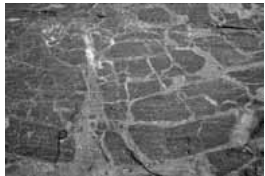
Figure 24 - Veining of a mafic dike by more evolved magma. The horizontal lines are glacial stripes.
