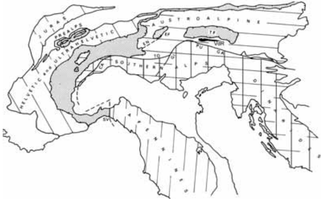
Figure 2 - Main Structural and paleogeographical domains of the Alps (from Dal Piaz et al., 1975).
