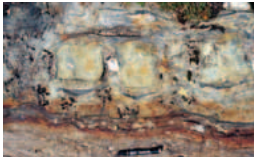
Figure 33 - Boudinage of a dm-thick amphibolite layer at the northern intrusive contact of the Vedrette di Ries tonalite, in the upper Val Sorgiva.
