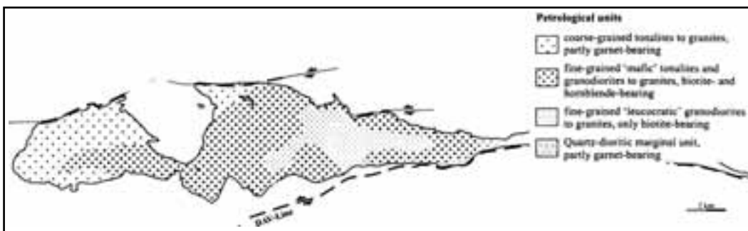
Figure 11 - Distribution of the various magmatic suites in the Vedrette di Ries Pluton (from Steenken et al. 2000).
