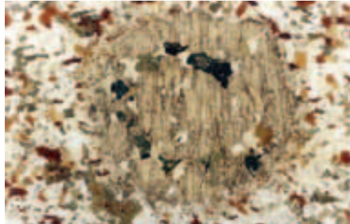
Figure 28 - Subhedral garnet with atoll inclusions (amphibole \pm plagioclase \pm biotite \pm opaque minerals), surrounded by a thin reaction rim.
