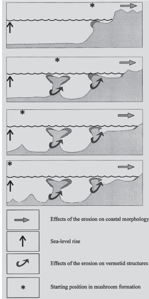
Figure 10 - Outline of the mechanisms of the mushroom-like Dendropoma concretionioning. Light grey rightward arrows indicate the effects of erosion on coastal morphology. Black arrow upward points out the sea-level rise. Symbol * marks the starting position in mushroom formation (from Antonioli et al., 1999).
