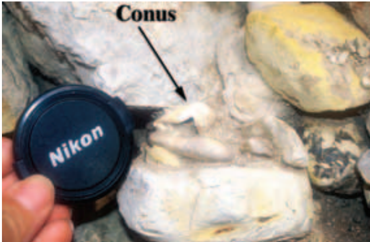
Figure 15 - Marine conglomerate, particular of the fossil that provided and ESR age for MIS 5.
