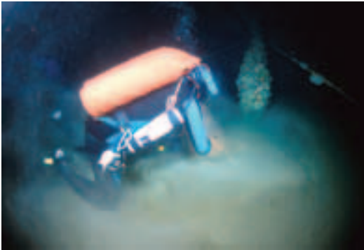
Figure 4 - A submerged cave at -30 m on the St. Vito Promontory showing a stalagmite with serpulids overgrowth.
