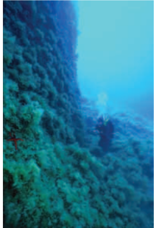
Figure 6 - The inner margin of a submerged terrace well carved between -15\18 m around all St. Vito Promontory.
