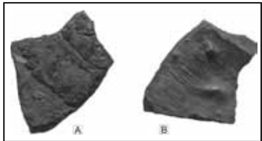
Figure 1 Stop 2 - Sample of Etruscan-Roman smelting scoria; A) upper surface; B) bottom surface.
