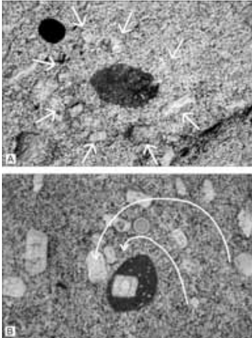
Figure 3 Stop 5 - A) Corona of K-feldspar megacrysts around a MME; B) vortex-like flow path followed by K-feldspar megacrysts around a MME. In (B) note the resorption texture of the K-feldspar megacryst within MME.
