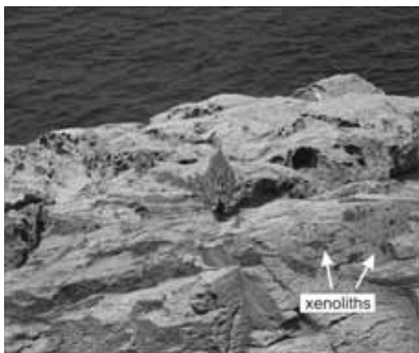
Figure 2 Stop 10 - “Leopard skin” aspect of the xenoliths-rich fine-grained facies
