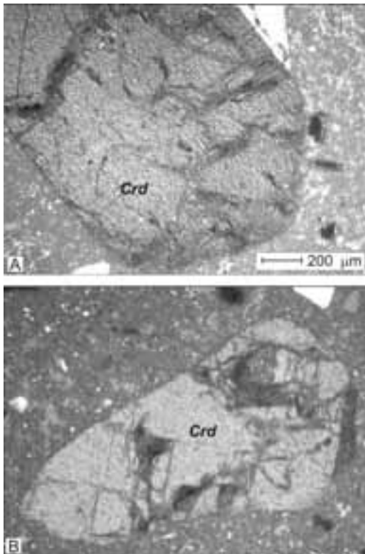
Figure 4 Stop 14 - A) and B) phenocrysts of cordierite having euhedral-subhedral and anhedral morphology, respectively.
