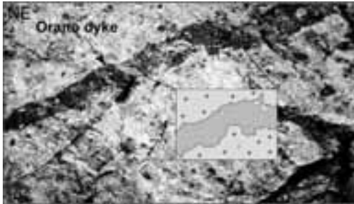
Figure 1 Stop 7 - Detail of the Orano dykes. Note the presence of both sharp and crenulated contacts along the margins of the dyke, as well as the re-orientation of corroded K-feldspar megacrysts within the dyke.
