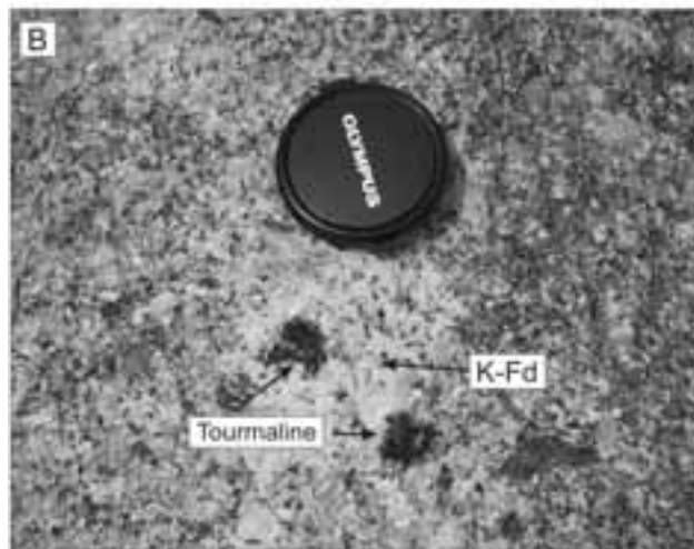
Figure 4 Stop 10 - A) Coarse-grained leucocratic facies of the Giglio Porto granitoid showing large poikilitic crystals of K-feldspar; B) large crystal of K-feldspar occurring in the leucocratic facies including nodules of tourmaline.
