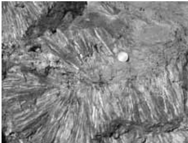
Figure 1 Stop 12 - Detailed view of hedenbergite radiate crystals belonging to the skarns occurring in the area of Temperino mine.
