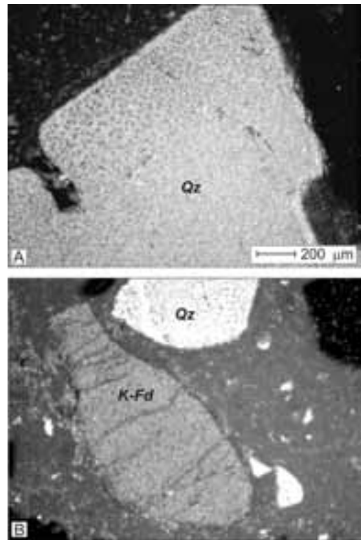
Figure 5 Stop 14 - Examples of crystals showing disequilibrium textures; A) crystal of quartz with embayments; B) corroded crystals of quartz (upper part) and K-feldspar (sanidine).
