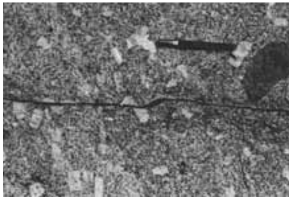
Figure 2 Stop 9 - Globular masses of darker Montecristo monzogranite (maximum dimension 10 m) in the more typical paler variety (Cala Giunchitelli).
