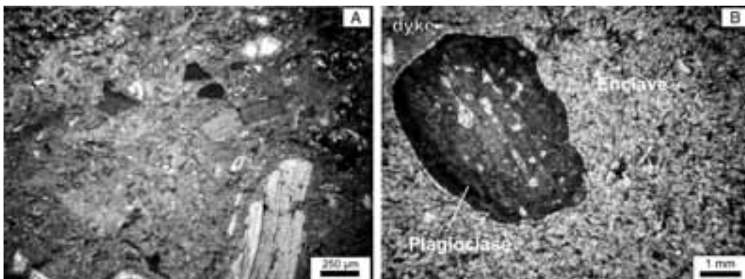
Figure 3 Stop 7 - (A): fine-grained fluidal porphyritic texture of the Orano dyke with biotite phenocrysts; (B) "dusty" plagioclase phenocryst cutting across the dyke/enclave interface.
