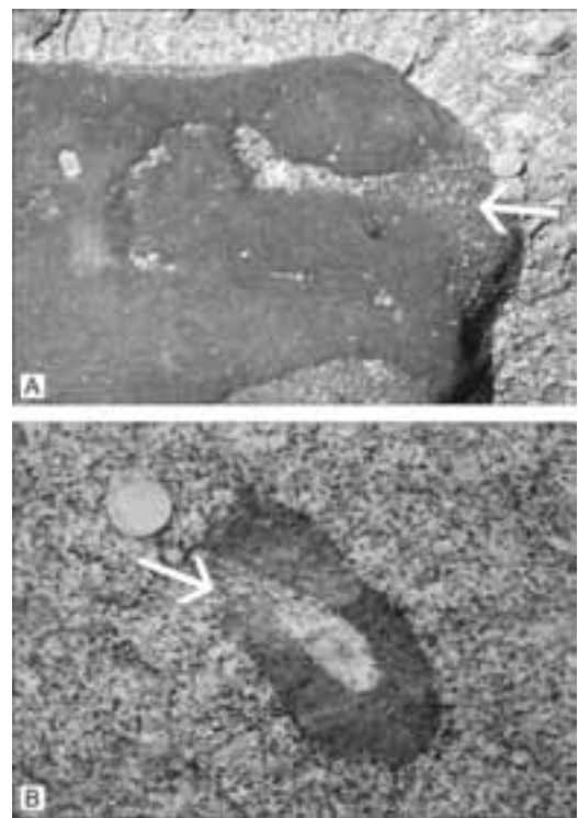
Figure 2 Stop 5 - A-B) Transfer of leucocratic material from the host magma to the MME by infiltration channels. In (B) the presence of a K-feldspar megacryst in the MME at the end of the infiltration channel indicates that it has been responsible for the disruption of the enclave boundary allowing the host magma to infiltrate.
