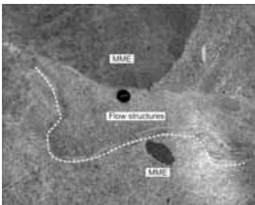
Figure 2 Stop 4 - Coexistence of Mafic Microgranular Enclaves (MME) and flow structures generated by the intimate dispersion of the mafic magma through the acid one.
