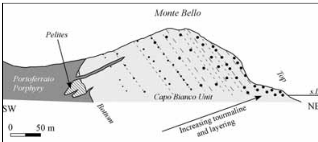
Figure 3 Stop 1 - Schematic section of Capo Bianco outcrop showing the increase of tourmaline spots size toward the top of the intrusion.
