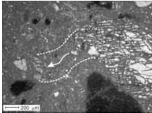
Figure 3 Stop 14 - Schlieren-like structure generated by the disruption of a K-feldspar (sanidine) phenocryst; dashed lines and arrow indicate the possible direction of the flow.
