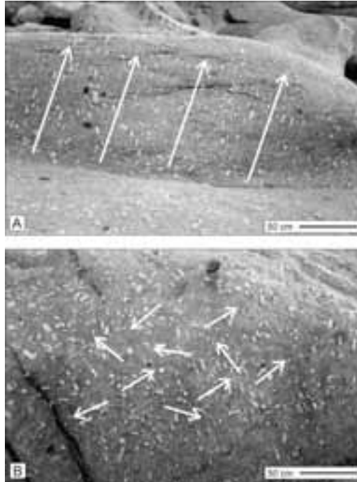
Figure 4 Stop 5 - Different flow fields at Sant'Andrea outcrop evidenced by the orientation of K-feldspar megacrysts. A) laminar flow field; B) random flow field.
