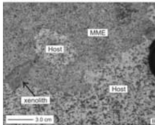
Figure 3 Stop 4 - A) Occurrence of two metamorphic xenoliths, one within a MME and the other sticking at the MME boundary; B) metamorphic xenolith passing from the host rock to the MME. The MME shown in (B) also contains a sub-spherical blob of host rock.
