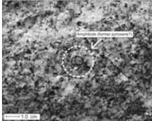
Figure 6 Stop 4 - Pseudomorphic crystal of amphibole evidenced in the picture by the dashed circle.
