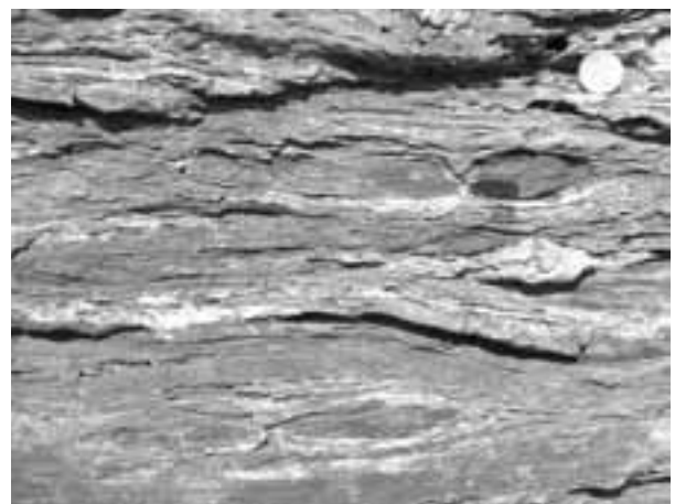
Figure 2 Stop 8 - Brittle deformation with formation of boudins of silicate-rich layers.
