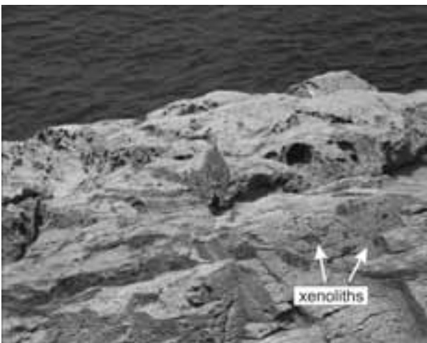
Figure 2 Stop 11 - “Leopard skin” aspect of the xenoliths-rich fine-grained facies.
