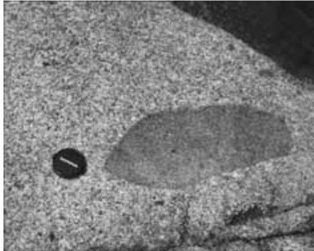
Figure 3 Stop 10 - Example of Mafic Microgranular Enclave (MME) with ovoid shape.
