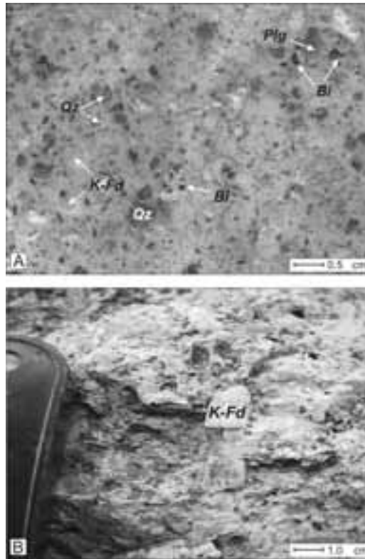
Figure 2 Stop 14 - A) Macroscopic view of a sample from Roccatederighi showing the glassy groundmass in which phenocrysts are immersed; B) detailed view of a sample from Roccatederighi showing the microcrystalline groundmass with the presence of K-feldspar (sanidine) megacrysts.
