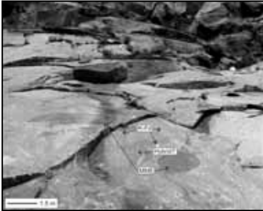
Figure 1 Stop 4 - General view of Pomonte quarry showing different magmatic interaction structures; MME=Mafic Microgranular Enclaves; Hybrid?=flow structures having a color index (mineralogical assemblage and grain size) intermediate between MME and the host granitoid mass. In the picture are also indicated K-feldspar (K-Fd) megacrysts.
