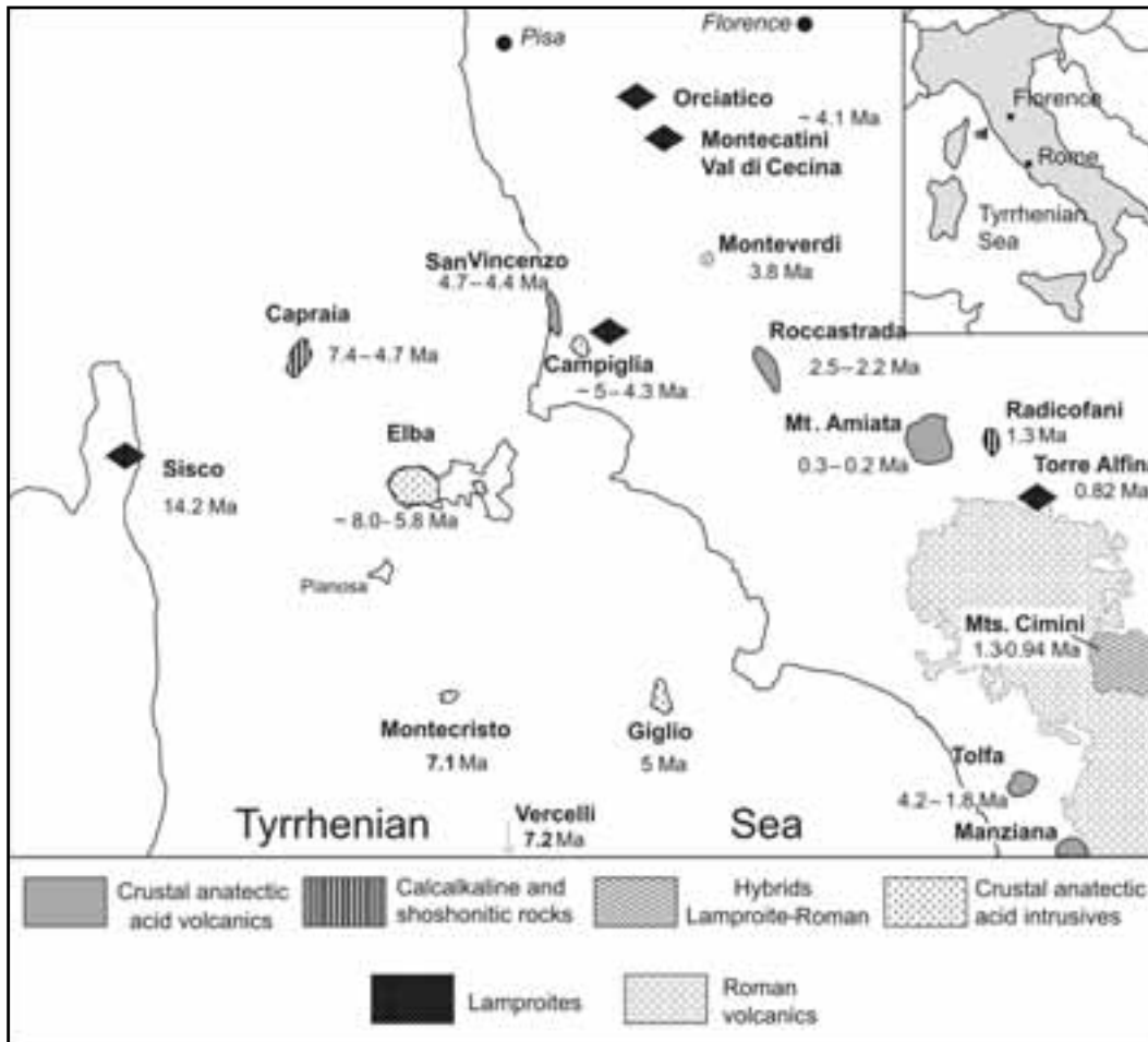
Figure 2 - Location, age and compositional characteristics of intrusive and extrusive rocks of the Tuscan magmatic province. Note the younging of magmatism from west to east.
