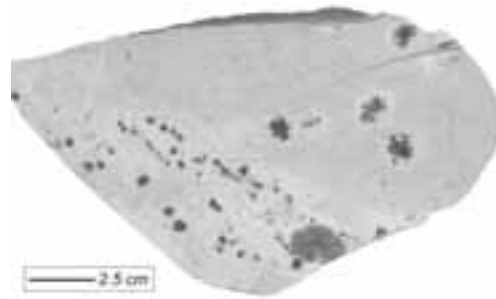
Figure 2 Stop 1 - Detail of a sample of the fine grained alkali feldspar granite containing black spots of tourmaline.
