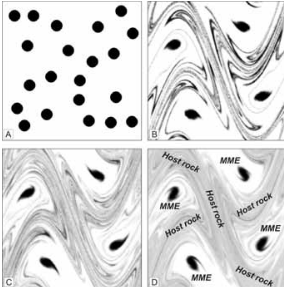
Figure 5 Step 4 - Example of chaotic mixing system whose evolution starts from the distribution of spherical blobs of mafic magma reported in (A) and moves on in time producing the mixing systems reported in (B), (C) and (D). Note in (D) the coexistence in space and time of completely hybridised portions of magmatic system (Host rock) and unmixed or poorly mixed sub-spherical blobs of mafic magma (MME) analogous to those observed in the Pomonte quarry outcrop.
