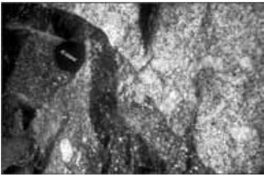
Figure 2 Stop 7 - Detail of a host/dyke contact in a Orano dyke. Note the abundance of plagioclase phenocrysts in the dyke and the presence of K-feldspar megacrysts in both the dyke and host, and the dyke cutting across one megacryst of the host.
