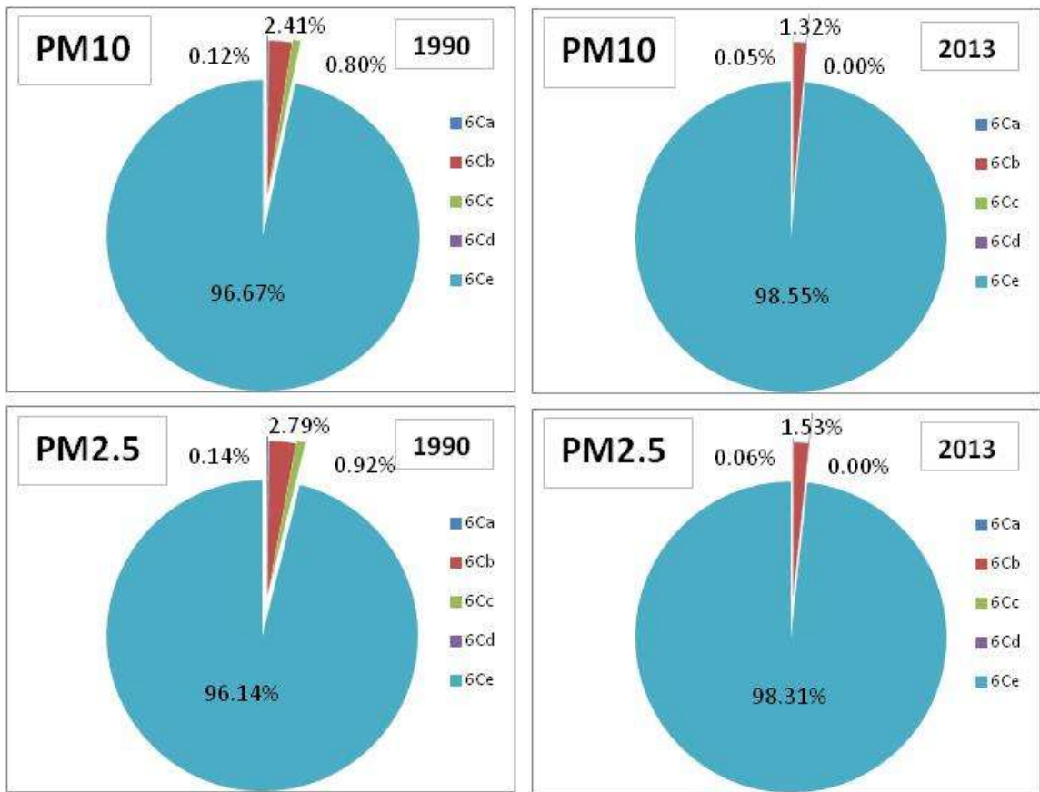
Figure 7.4 Contribution of PM10 and PM2.5 sub-category emissions to waste sector total emissions
