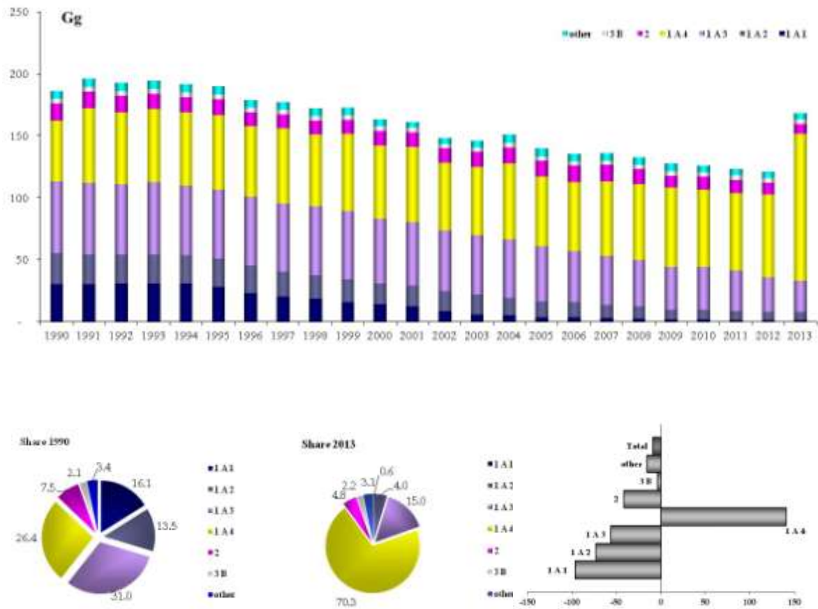
Figure 2.7 PM2.5 emission trend, percentage share by sector and variation 1990-2013
