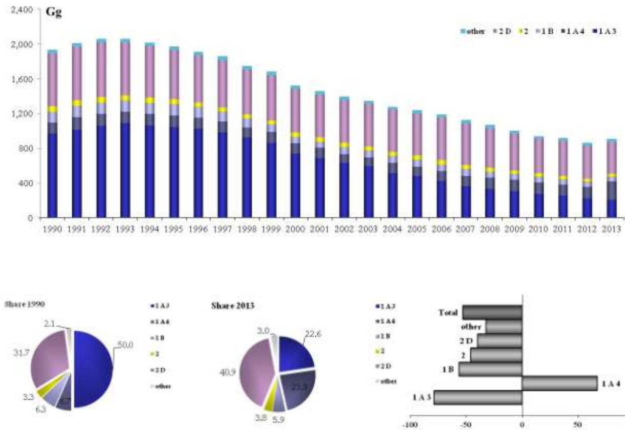
Figure 2.4 NMVOC emission trend, percentage share by sector and variation 1990-2013
