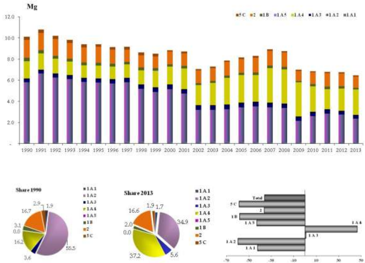
Figure 2.10 Cd emission trend, percentage share by sector and variation 1990-2013
