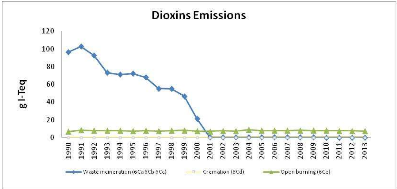
Figure 7.5 Time series of dioxin emissions of the waste sector by category (g I-Teq)
