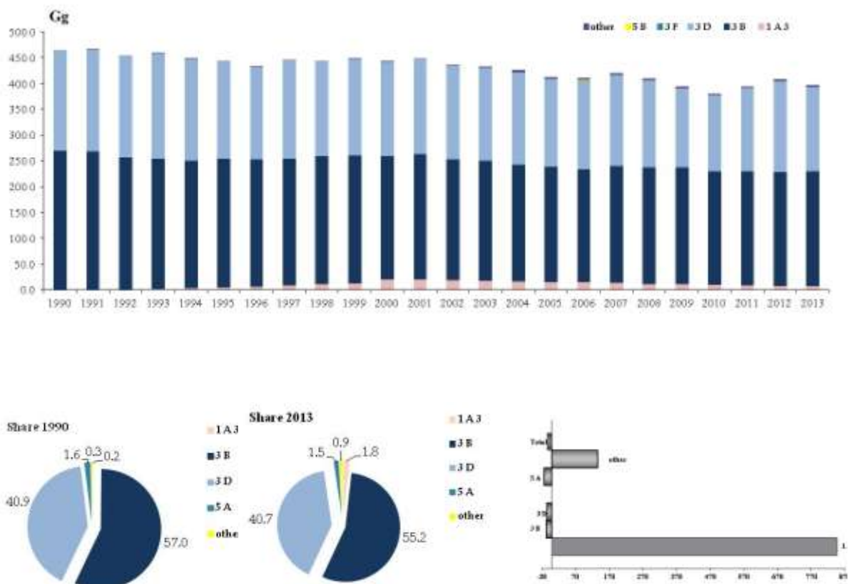
Figure 2.3 NH 3 emission trend, percentage share by sector and variation 1990-2013
