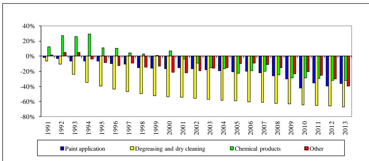
Figure 5.2 Trend of NMVOC emissions from 1991 to 2013 as compared to 1990
