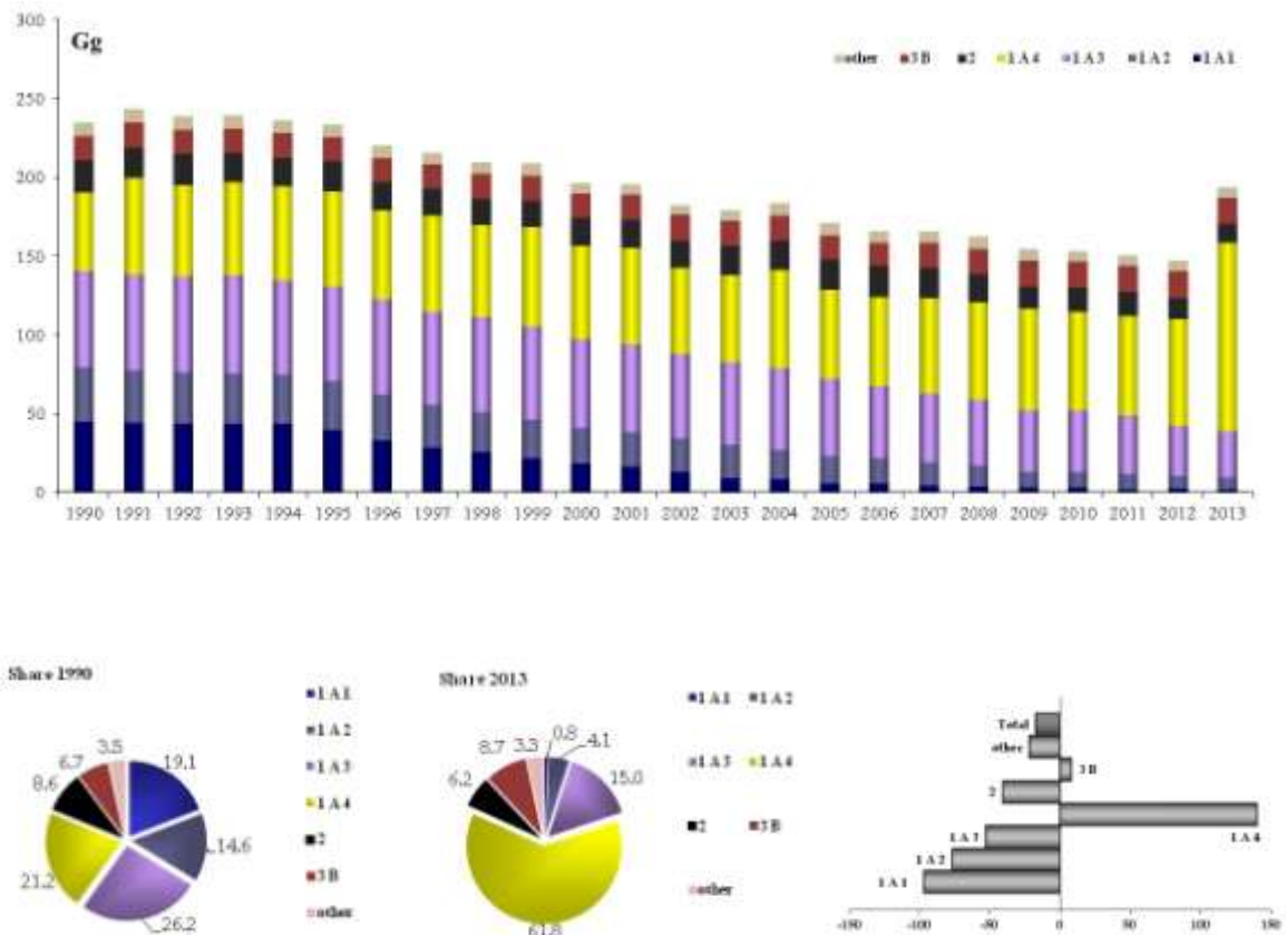
Figure 2.6 PM10 emission trend, percentage share by sector and variation 1990-2013
