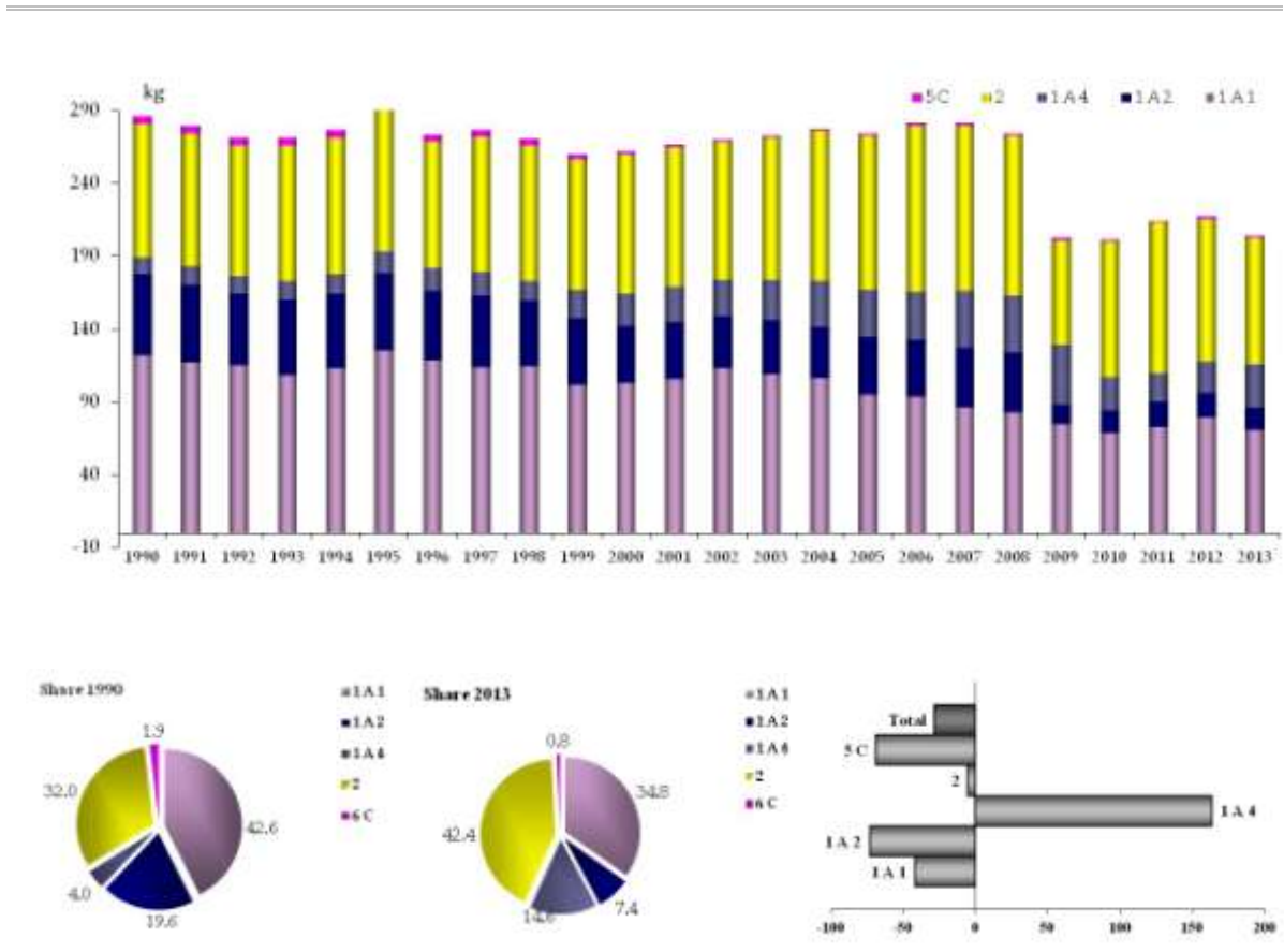
Figure 2.15 PCB emission trend, percentage share by sector and variation 1990-2013
