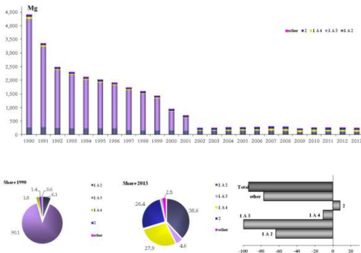
Figure 2.9 Pb emission trend, percentage share by sector and variation 1990-2013
