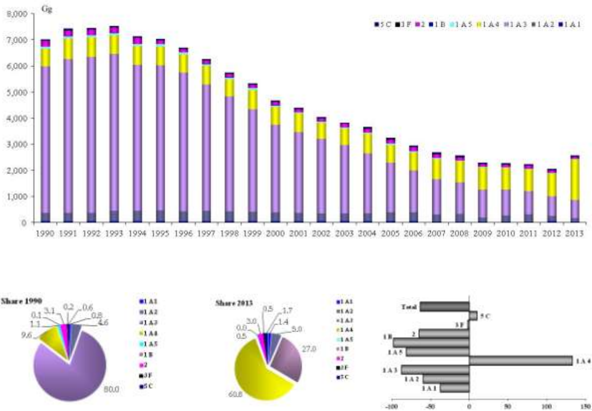
Figure 2.5 CO emission trend, percentage share by sector and variation 1990-2013
