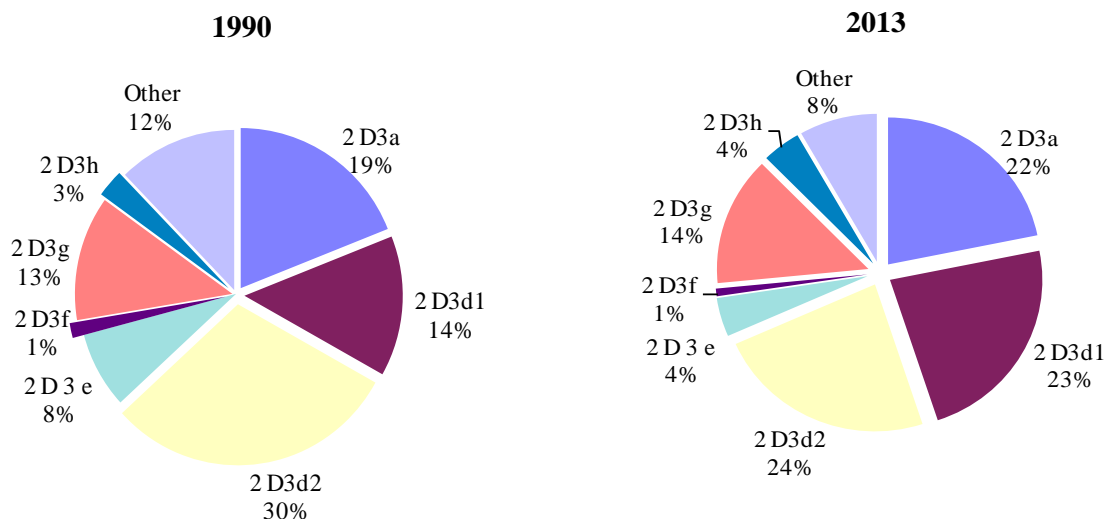
Figure 5.1 Share of NMVOC emissions for the solvent use sector in 1990 and 2013
