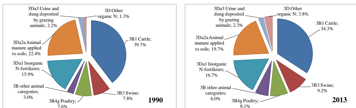
Figure 6.1 Share of NH 3 emissions in the agriculture sector for 1990 and 2013
