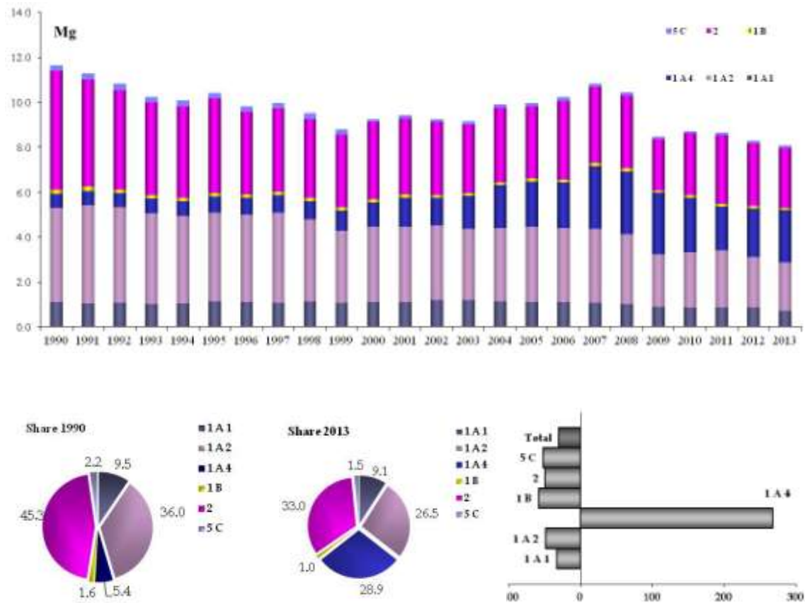
Figure 2.11 Hg emission trend, percentage share by sector and variation 1990-2013
