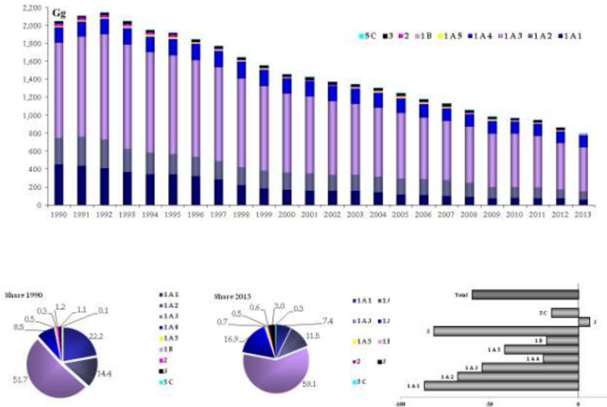
Figure 2.2 NO x emission trend, percentage share by sector and variation 1990-2013
