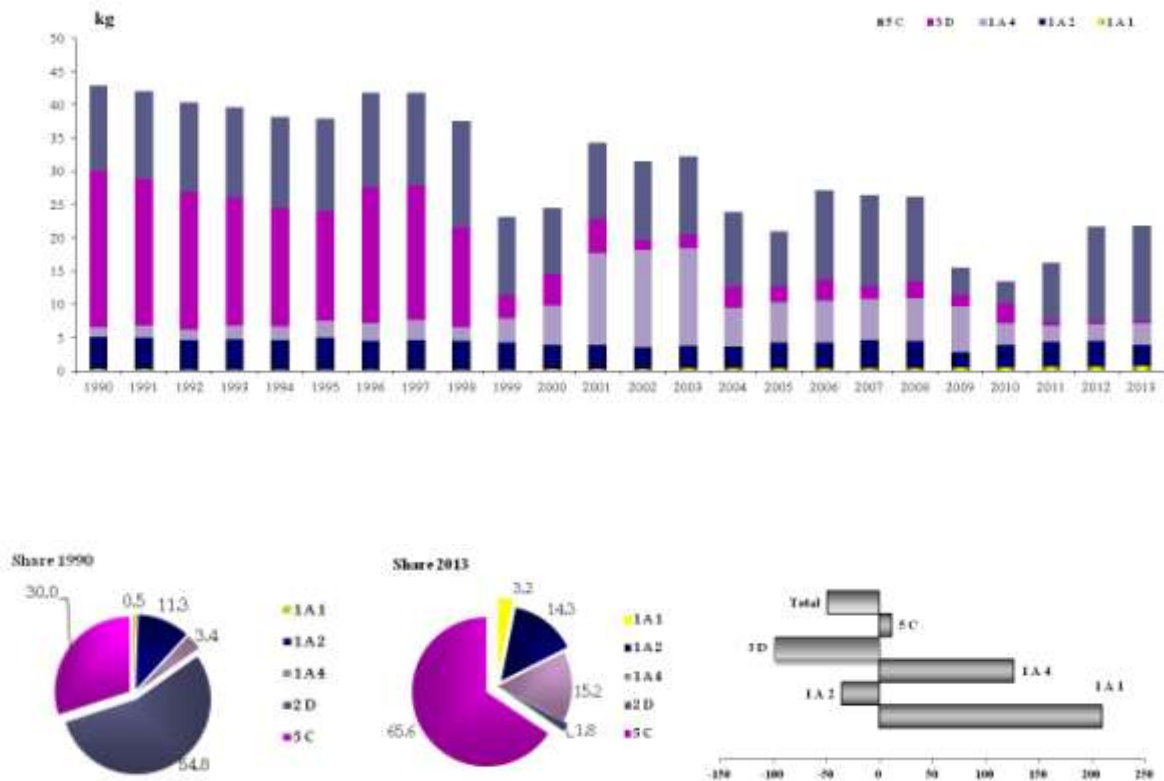
Figure 2.14 HCB emission trend, percentage share by sector and variation 1990-2013
