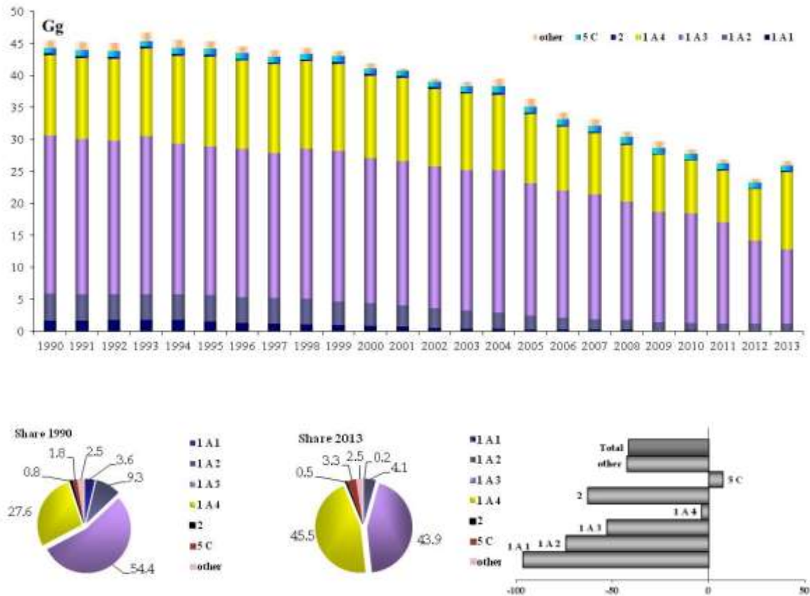
Figure 2.8 BC emission trend, percentage share by sector and variation 1990-2013
