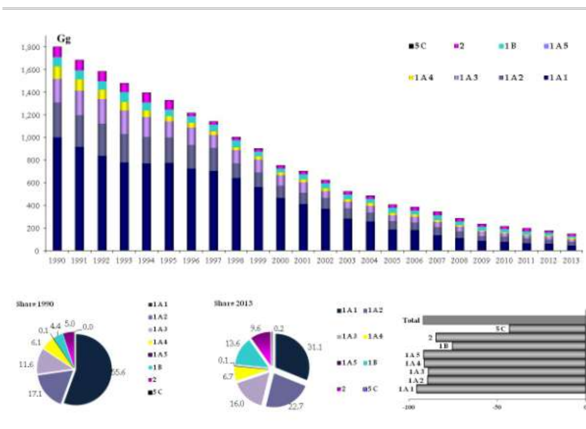
Figure 2.1 SO x emissions trend, percentage share by sector and variation 1990-2013
