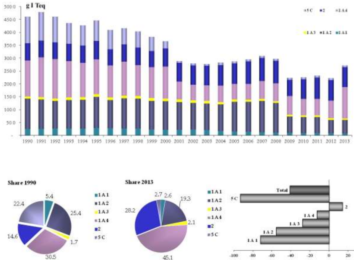
Figure 2.13 Dioxin emission trend, percentage share by sector and variation 1990-2013
