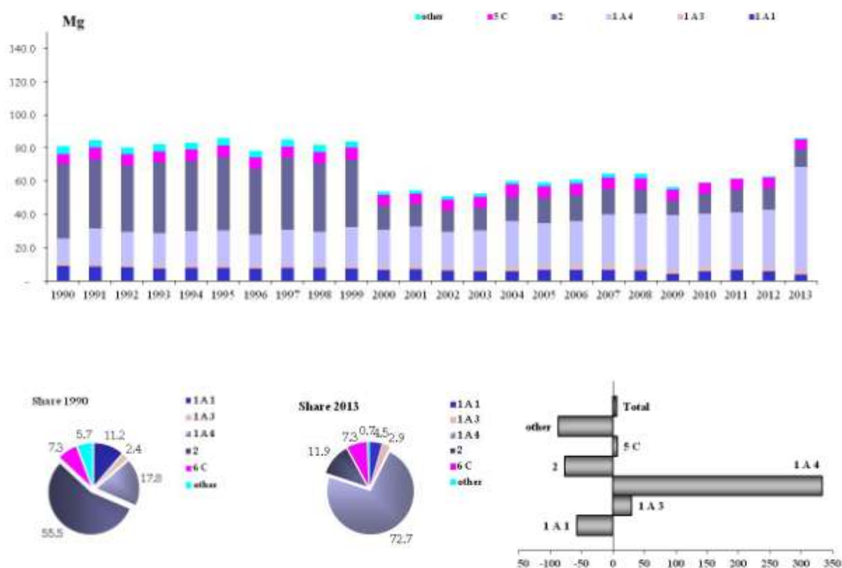
Figure 2.12 PAH emission trend, percentage share by sector and variation 1990-2013
