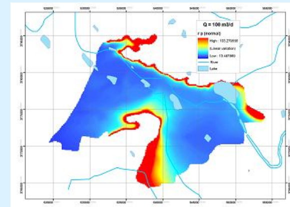
Protection distance perpendicular to flow direction (m)
