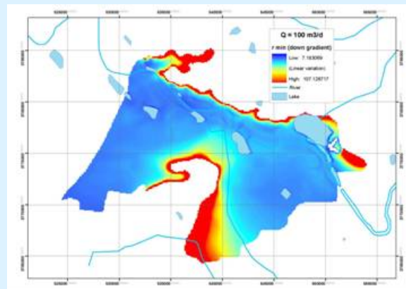
Downgradient protection distance (m)
