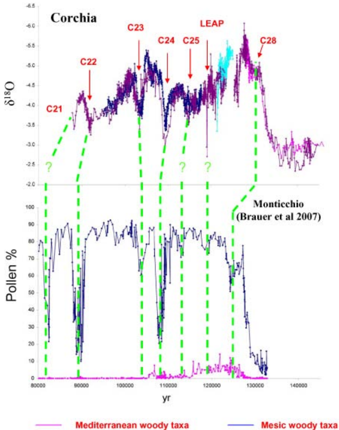
Fig. 3.13 - Comparison between the \delta^{18}O record from Corchia Speleothems (different colour means record obtained from different stalagmites; after Drysdale et al., 2009 and unpublished data) and Monticchio pollen record (Brauer et al., 2007). Cold event after McManus et al., 1994; 2006. LEAP: late-Eemian aridity pulse (Sirocko et al., 2005).
