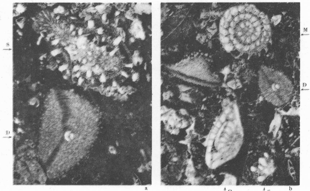
2 a & b : Miscellanea cf. miscella (D' ARCH.) (M), Discocyclusina cf. seunesi (H. Douv.) (D), Operculina sp. (O) e Siderolites calcitrapoides LAM. (S) in ciottoli.
